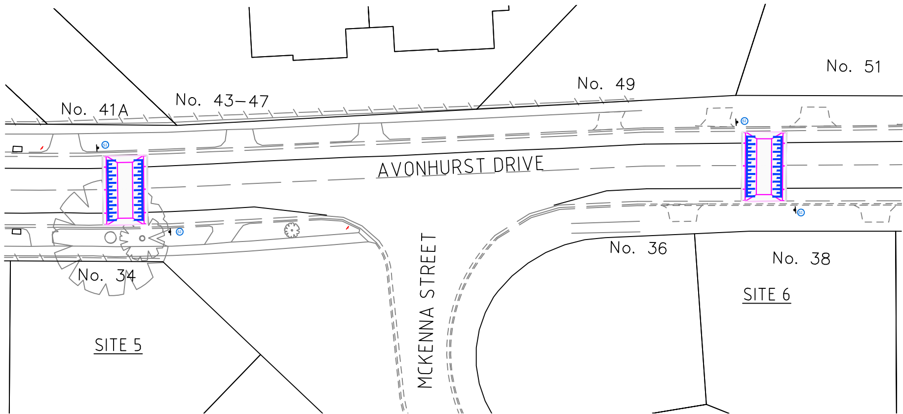
AVONHURST DRIVE ROAD HUMP & LINEMARKING PLAN
