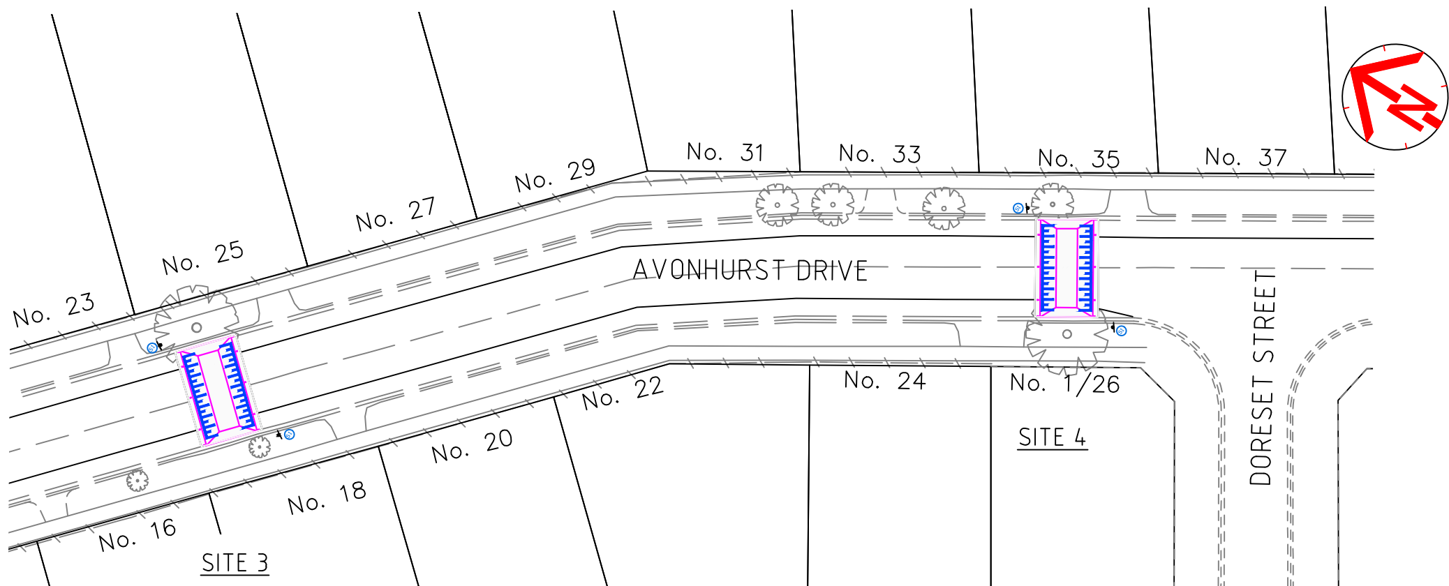
AVONHURST DRIVE ROAD HUMP & LINEMARKING PLAN
