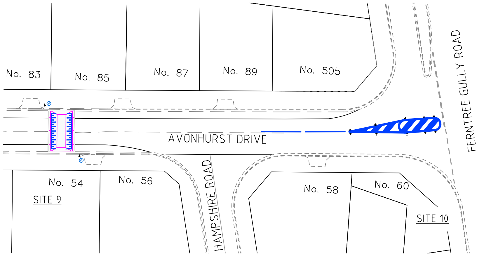
AVONHURST DRIVE ROAD HUMP & LINEMARKING PLAN
